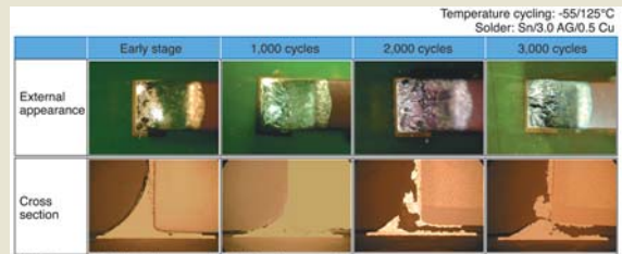
Note: The numerical values of the cross-section photographs are crack rates. Growth of solder cracks due to temperature cycling (page 16)
